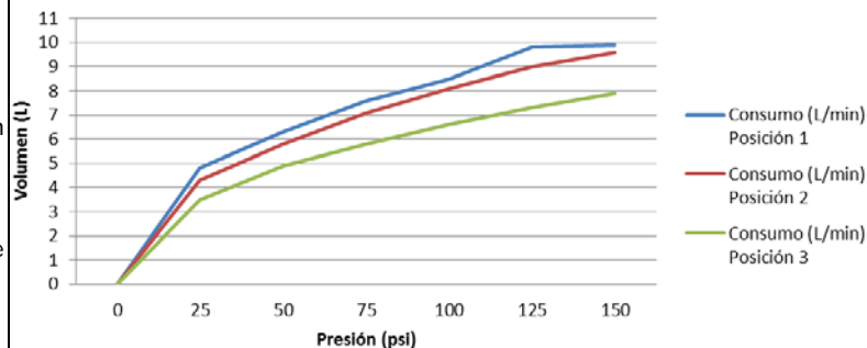
Consumo (L/min)
